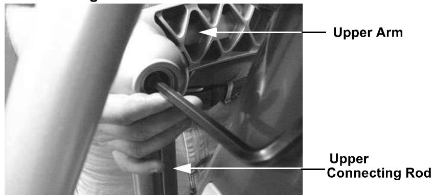
Diagram 7.29 - Upper Connecting Rod Removal
