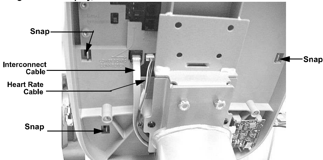
Diagram 7.1 - Display, with Rear Cover Removed
