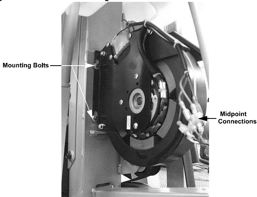
Diagram 7.8 - Generator Mounting
