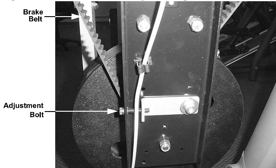
Diagram 5.3 - Brake Belt Idler Pulley Mounting Bolt
