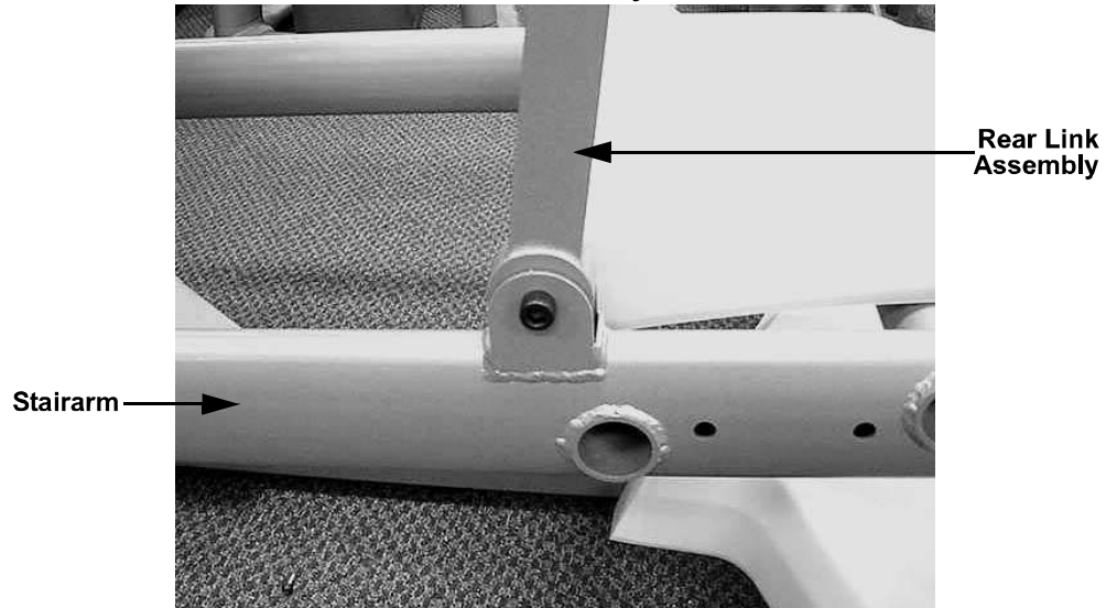
Diagram 7.9 - Stairarm and Rear Link Assembly
