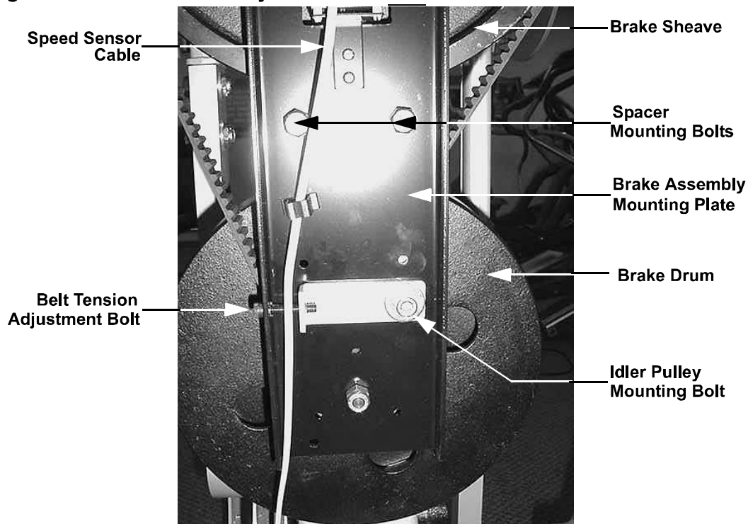
Diagram 7.5 - Brake Assembly
