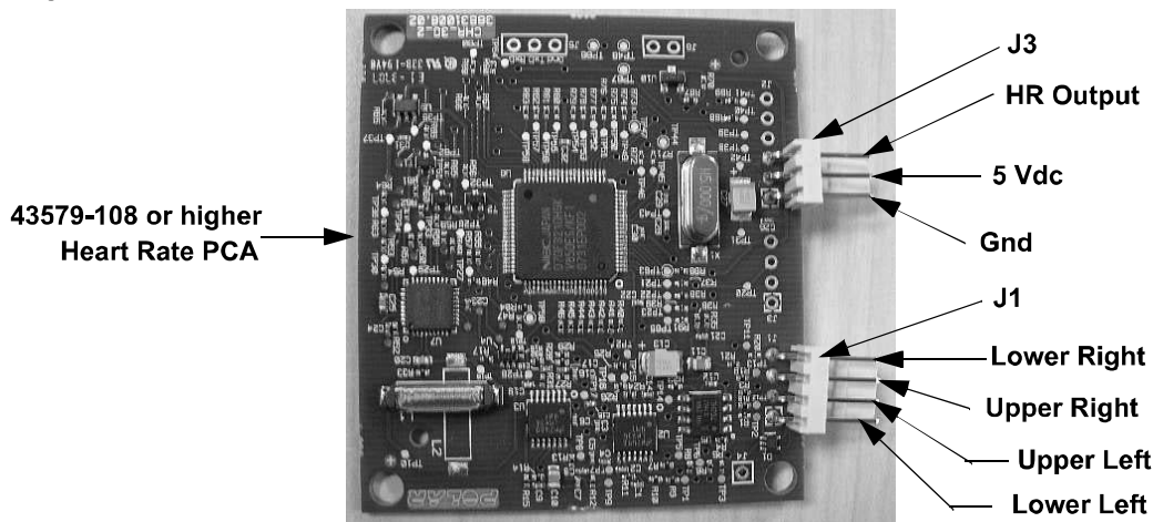
Diagram 6.3 - Hand held/chest strap heart rate PCA
