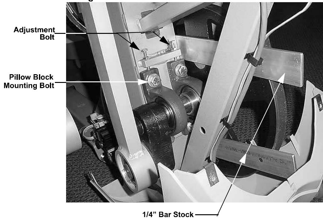
Diagram 5.4 - Drive Belt Alignment
