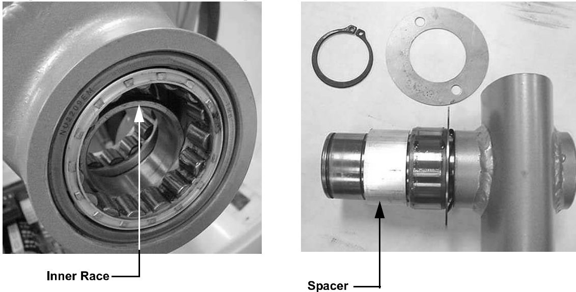
Diagram 7.11 - Front Brace Bearings
