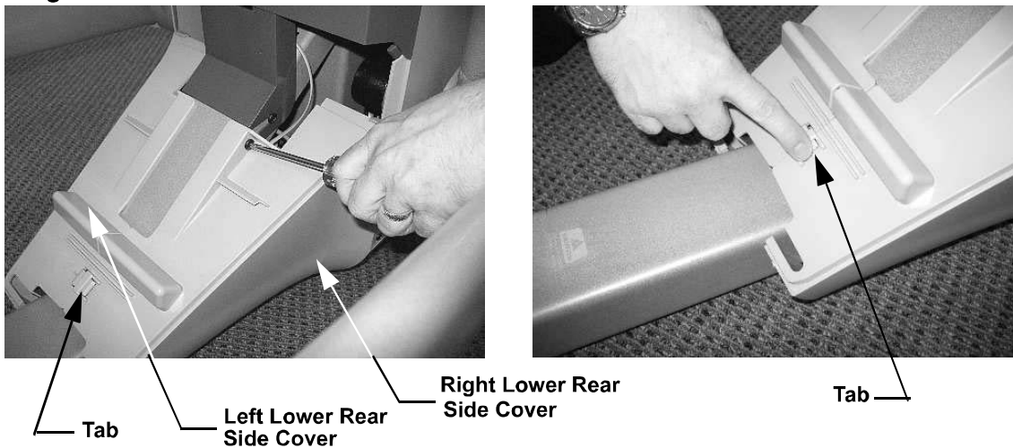
Diagram 7.17 - Lower Rear Side Covers
