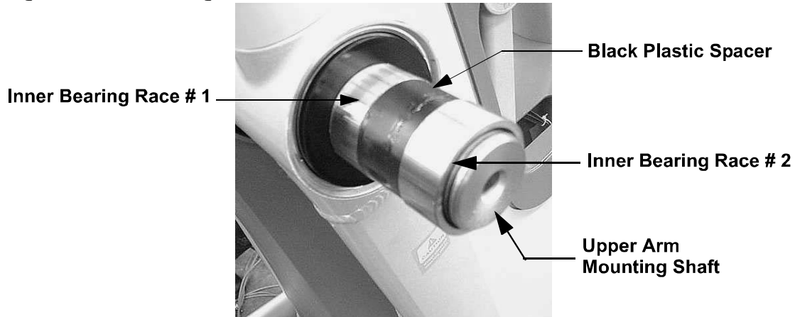
Diagram 7.30 - Bearing Removal.
