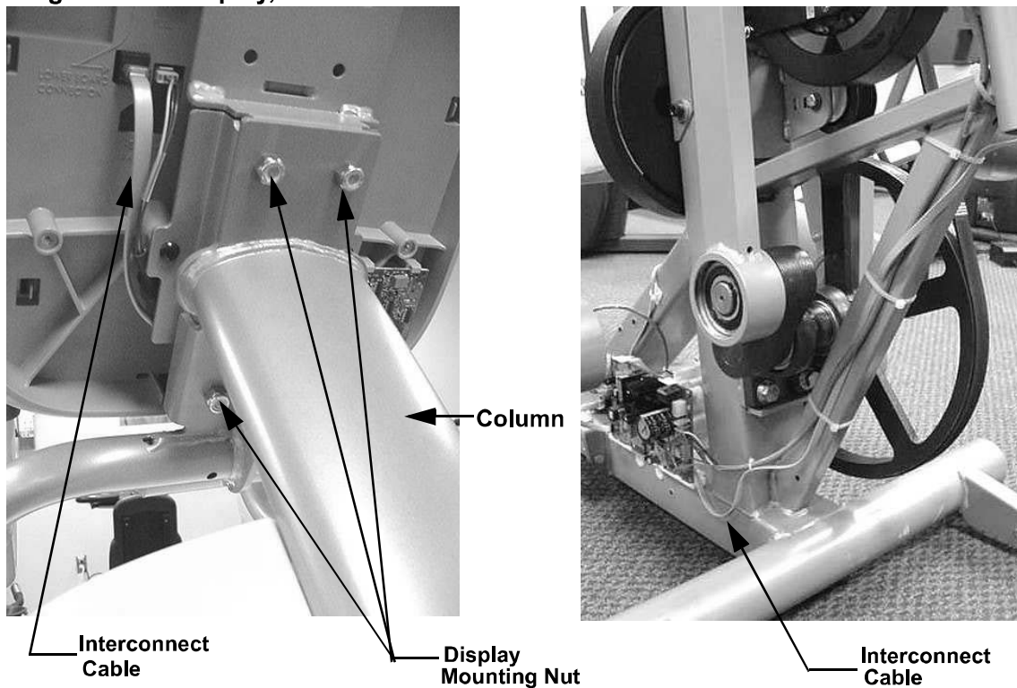
Diagram 7.3 - Display, Rear View
