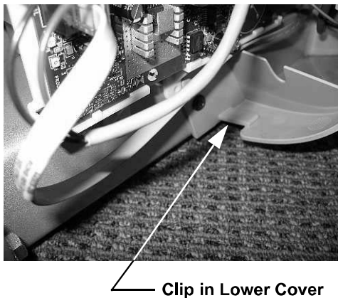
Diagram 7.22 - Lower Rear Side Covers
