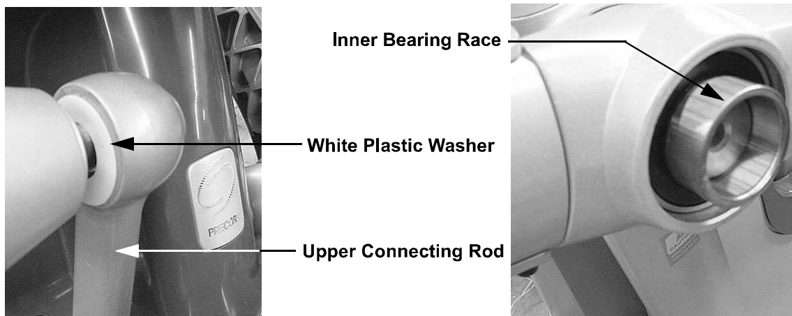
Diagram 7.31 - Bearing Replacement
