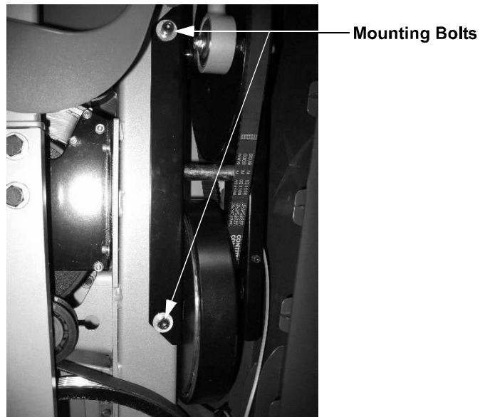
Diagram 7.14 - H-Brake Mounting Bolts
