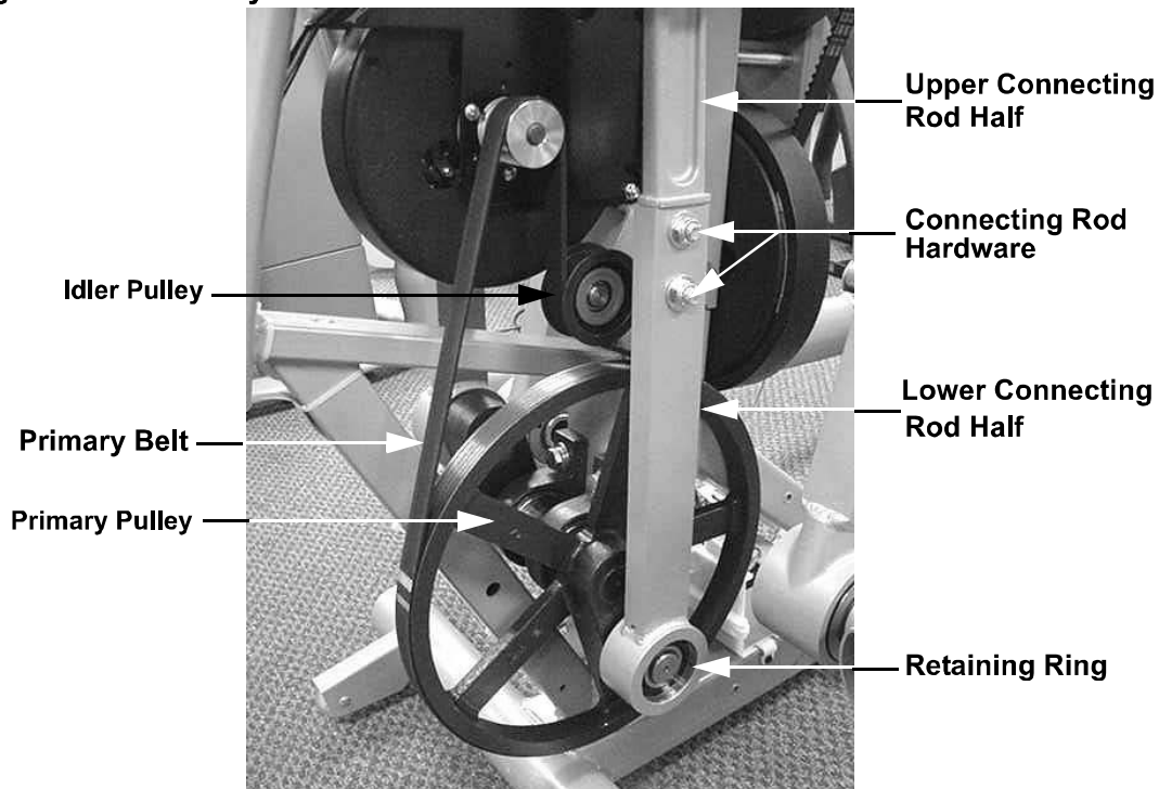
Diagram 7.4 - Primary Belt
