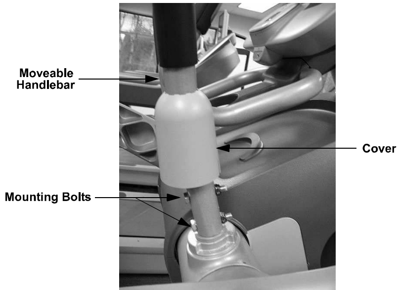
Diagram 7.32 - Moveable Handlebar
