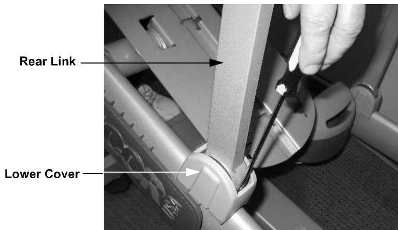
Diagram 7.25 - Releasing the Lower Cover
