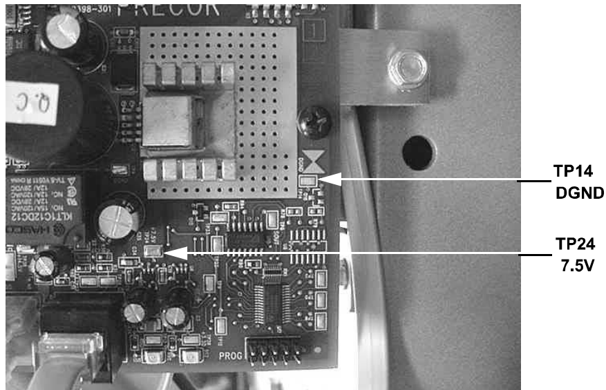
Diagram 6.2 - Partial View of Lower PCA
