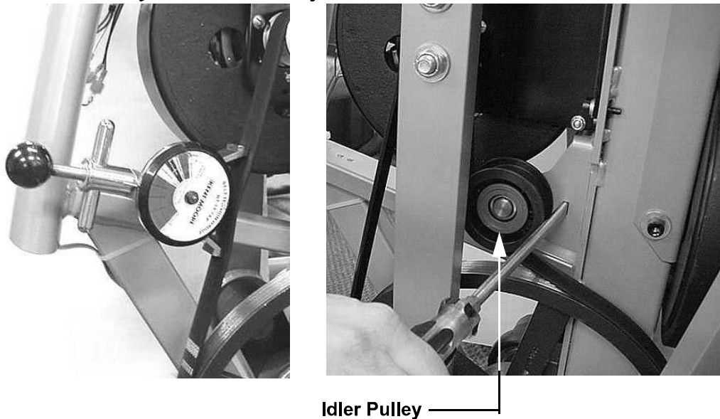
Diagram 5.2 - Primary Belt Tension Adjustment
