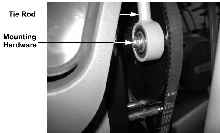
Diagram 7.12 - H-Brake Tie Rod Mounting
