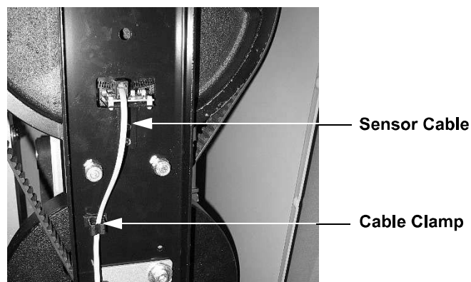
Diagram 7.13 - H-Brake Sensor Cable
